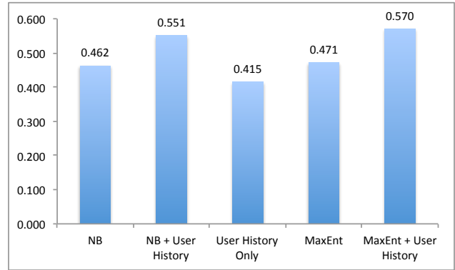
Figure 6. Classification accuracy with help of user check-in history
