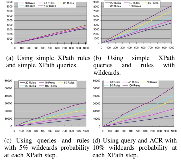
Fig. 10. System scalability: number of query segments.
